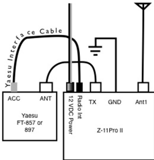
FT-857/897 Installation
